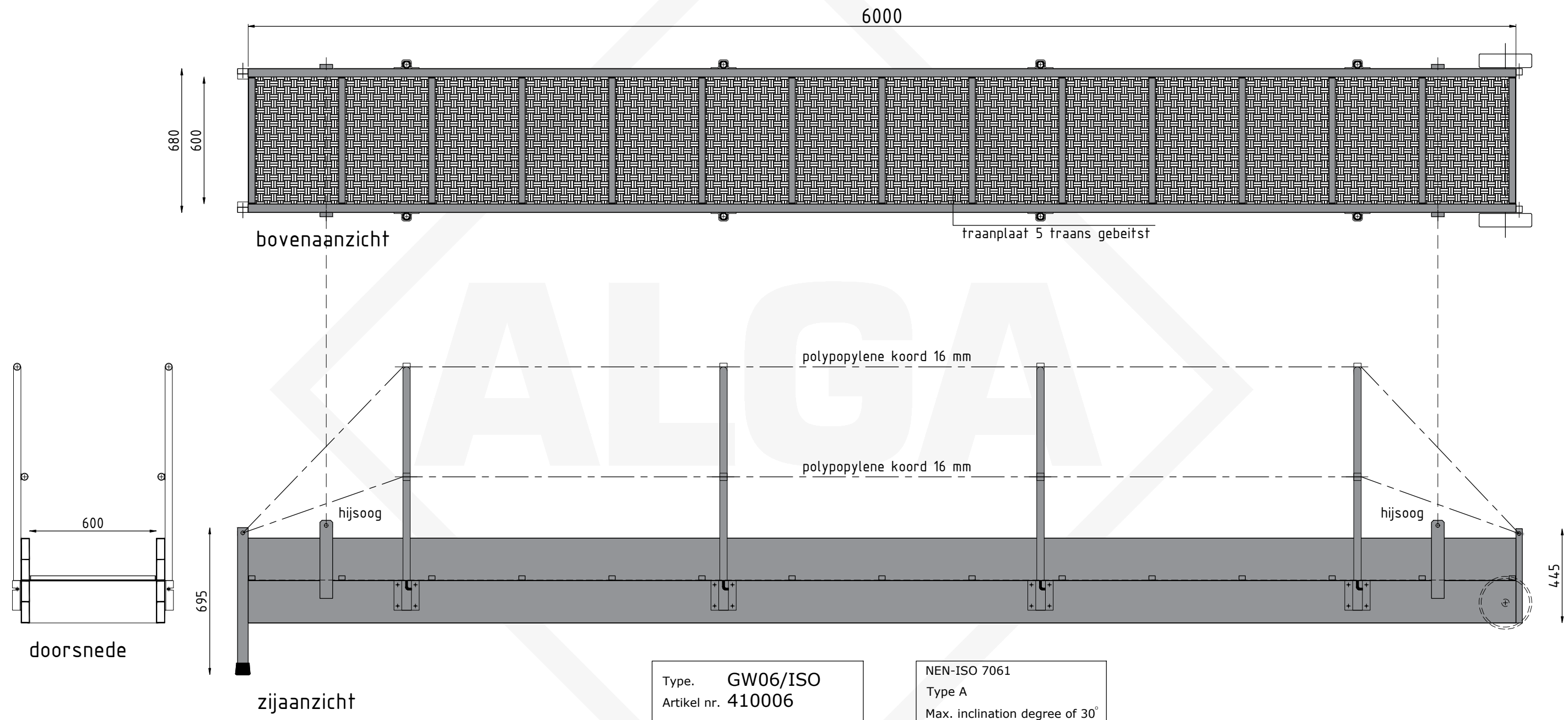
Aluminium gangway 6 meter ISO (Seagoing Vessels)
