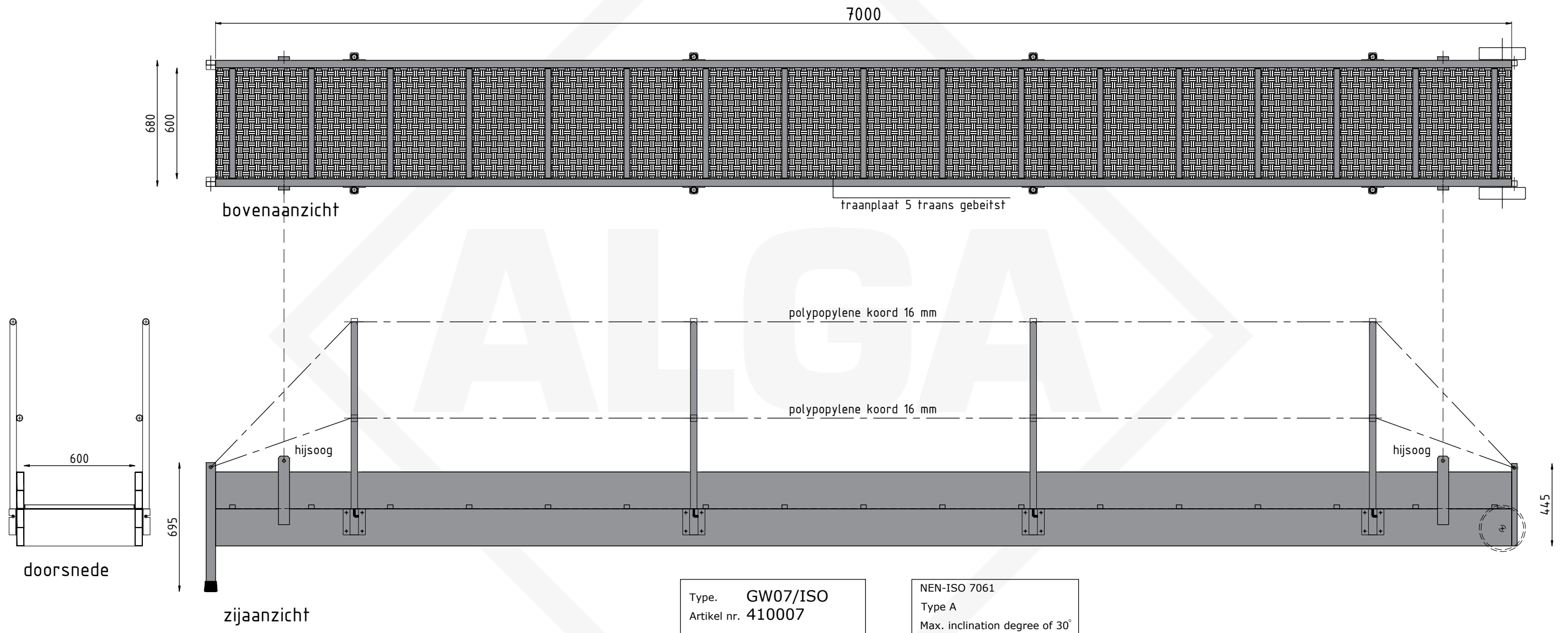
Aluminium gangway 7 meter ISO (Seagoing Vessels)
