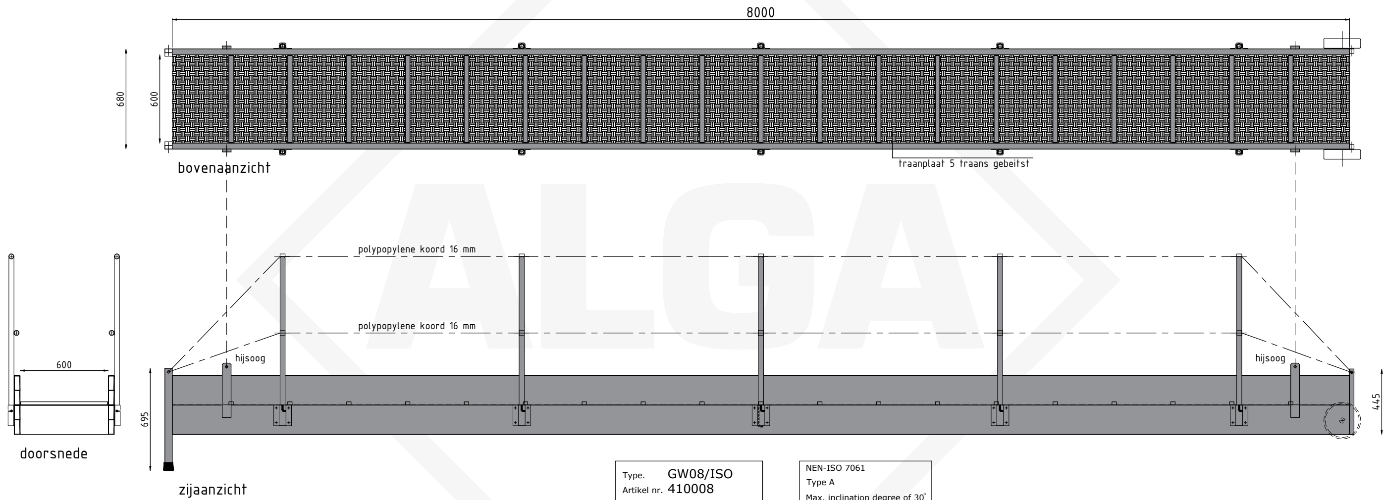
Aluminium gangway 8 meter ISO (Seagoing Vessels)
